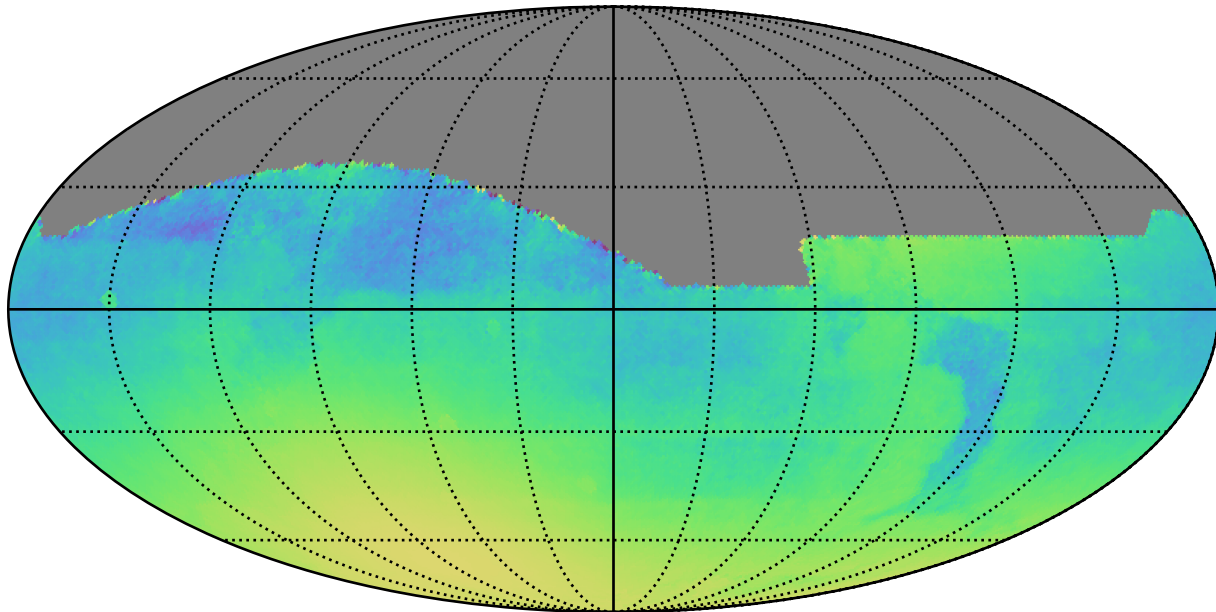
baseline_v3.3_10yrs All sky: Normalized Parallax Uncert @ 22.4
