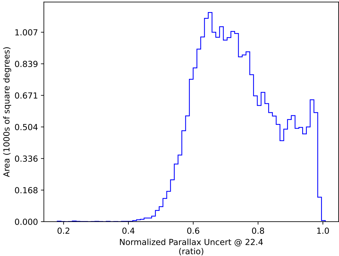
baseline_v3.3_10yrs All sky: Normalized Parallax Uncert @ 22.4
