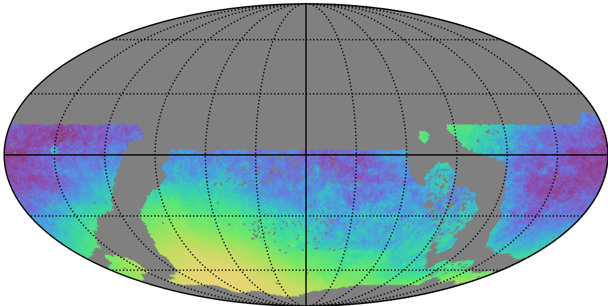
baseline_v3.3_10yrs WFD y band only: Normalized Parallax Uncert @ 21.3
