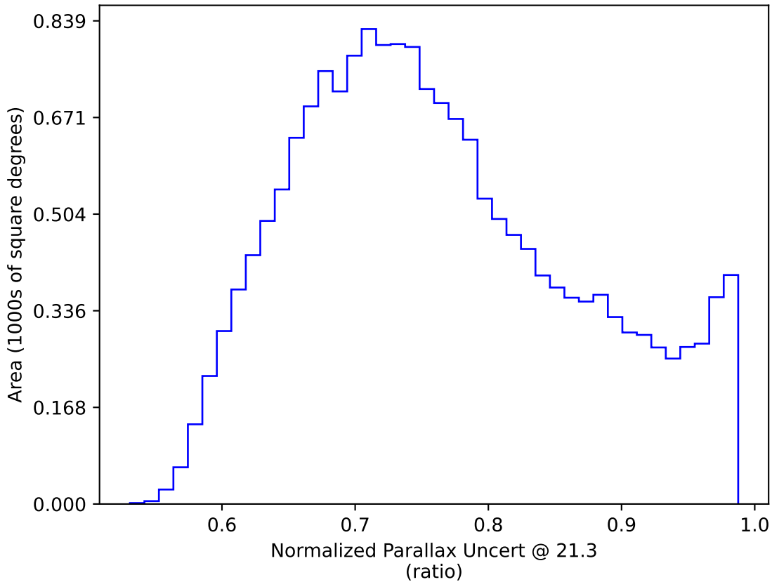
baseline_v3.3_10yrs WFD y band only: Normalized Parallax Uncert @ 21.3
