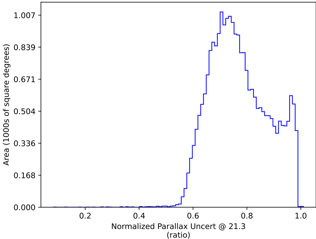
baseline_v3.3_10yrs All sky y band only: Normalized Parallax Uncert @ 21.3
