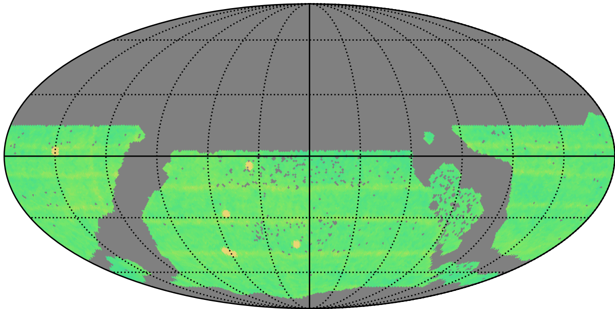
baseline_v3.3_10yrs WFD all bands: N Unique Nights
