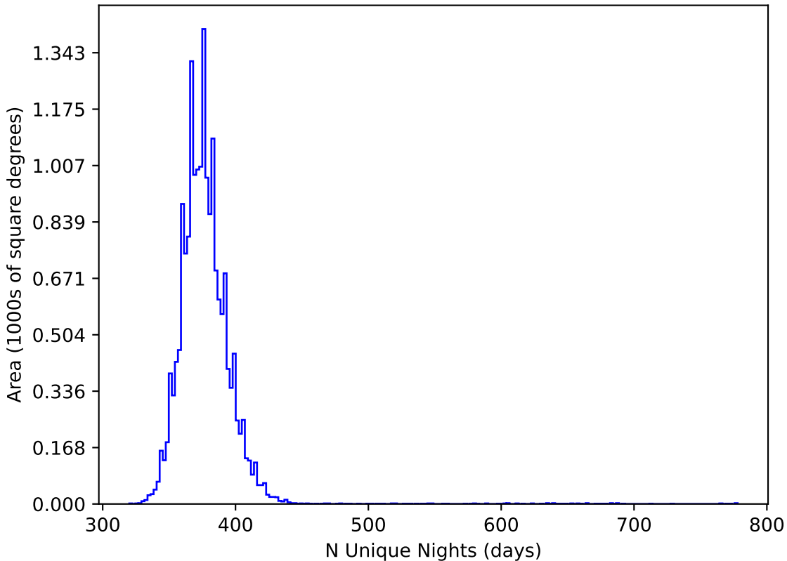
baseline_v3.3_10yrs WFD all bands: N Unique Nights
