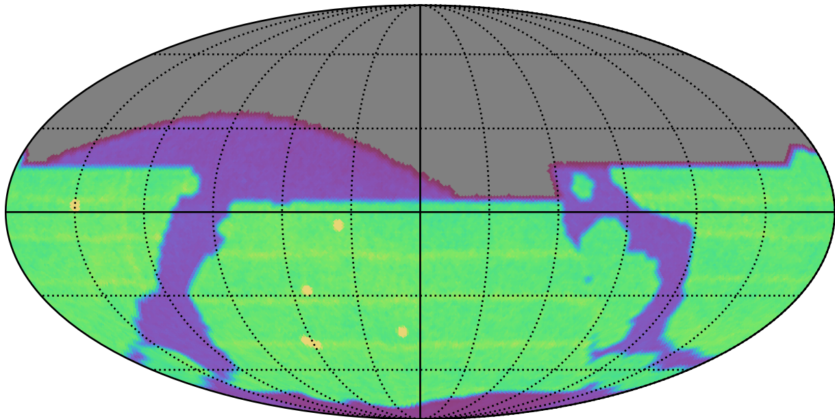
baseline_v3.3_10yrs All sky all bands: N Unique Nights
