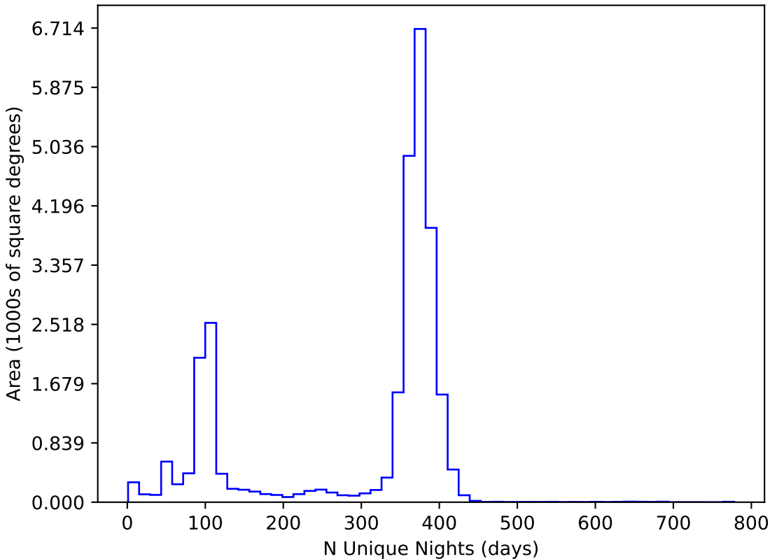
baseline_v3.3_10yrs All sky all bands: N Unique Nights
