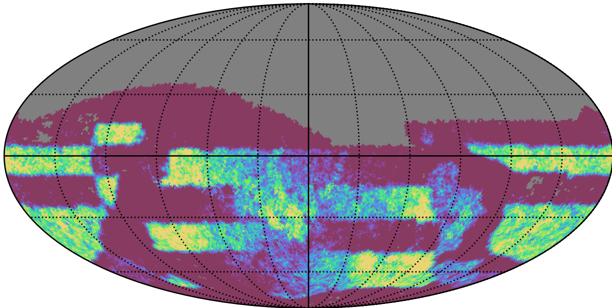
baseline_v3.3_10yrs Yr 3-4 z band: NVisits
