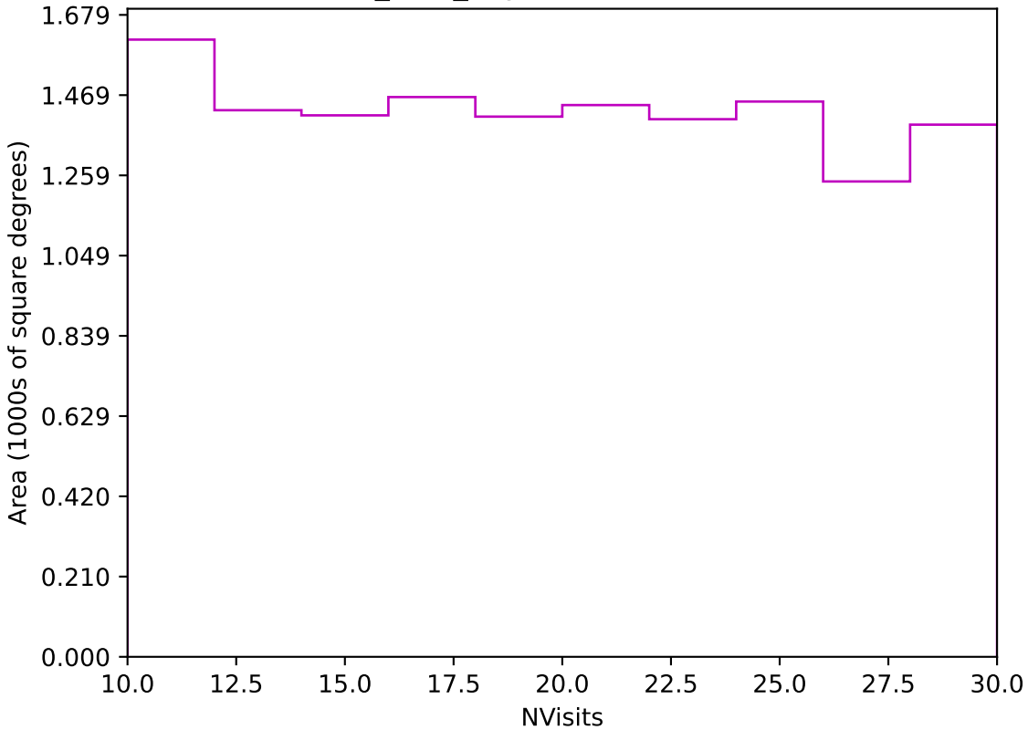
baseline_v3.3_10yrs Yr 3-4 z band: NVisits
