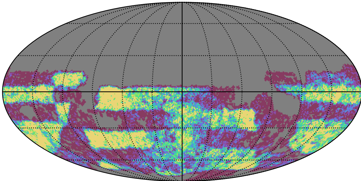
baseline_v3.3_10yrs Yr 3-4 u band: NVisits
