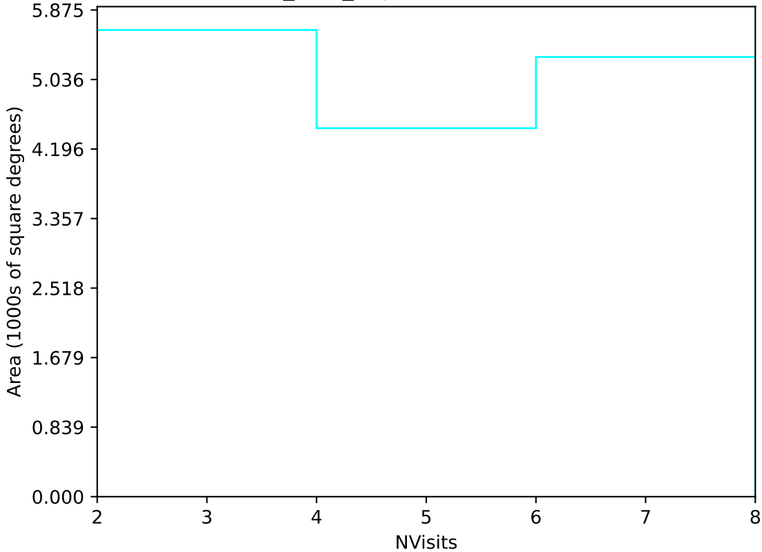
baseline_v3.3_10yrs Yr 3-4 u band: NVisits
