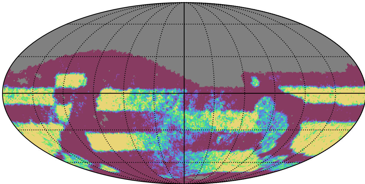
baseline_v3.3_10yrs Yr 3-4 r band: NVisits
