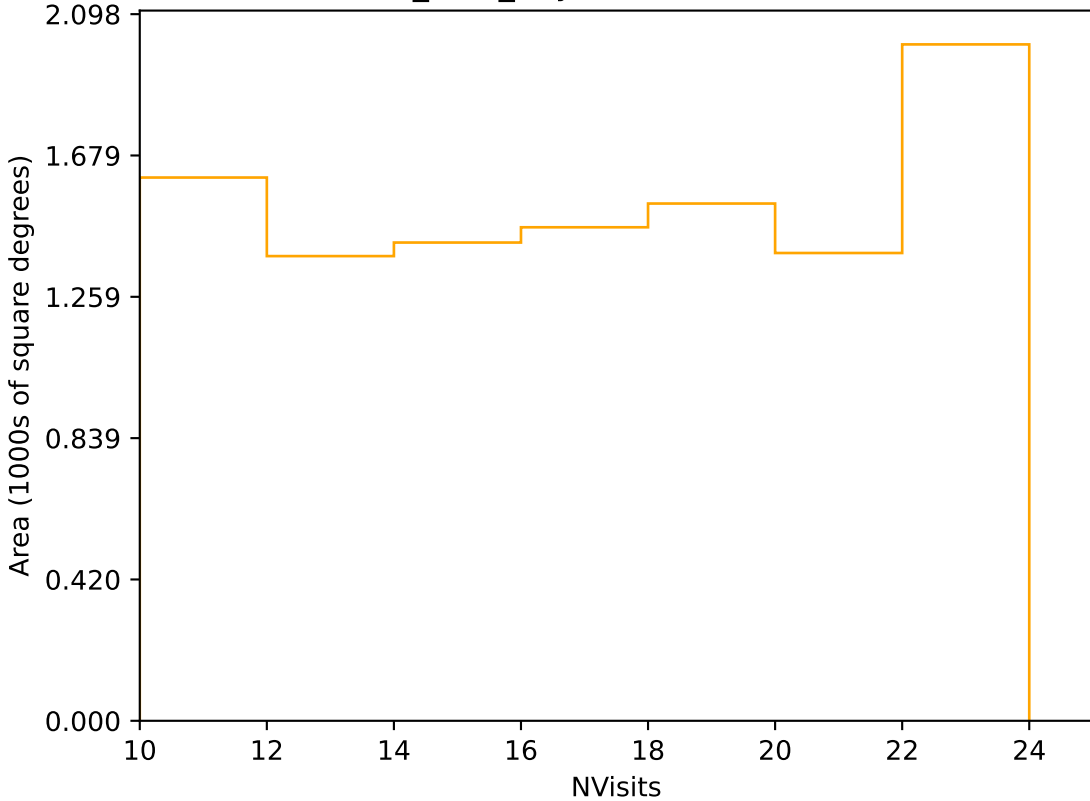
baseline_v3.3_10yrs Yr 3-4 r band: NVisits
