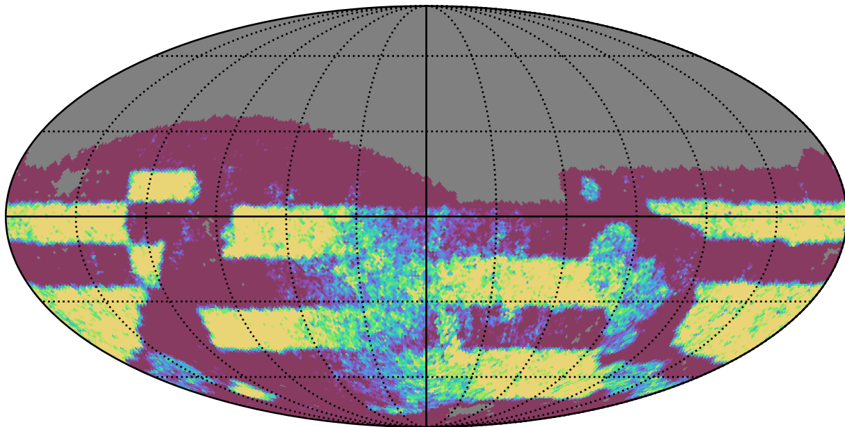
baseline_v3.3_10yrs Yr 3-4 i band: NVisits
