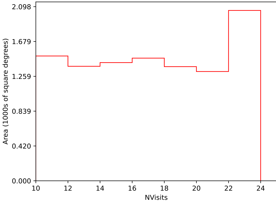
baseline_v3.3_10yrs Yr 3-4 i band: NVisits
