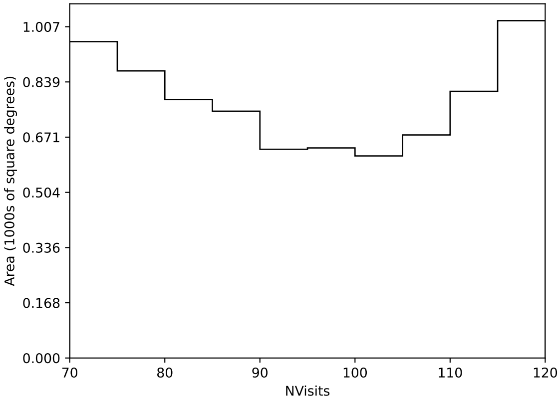
baseline_v3.3_10yrs Yr 3-4 all bands: NVisits
