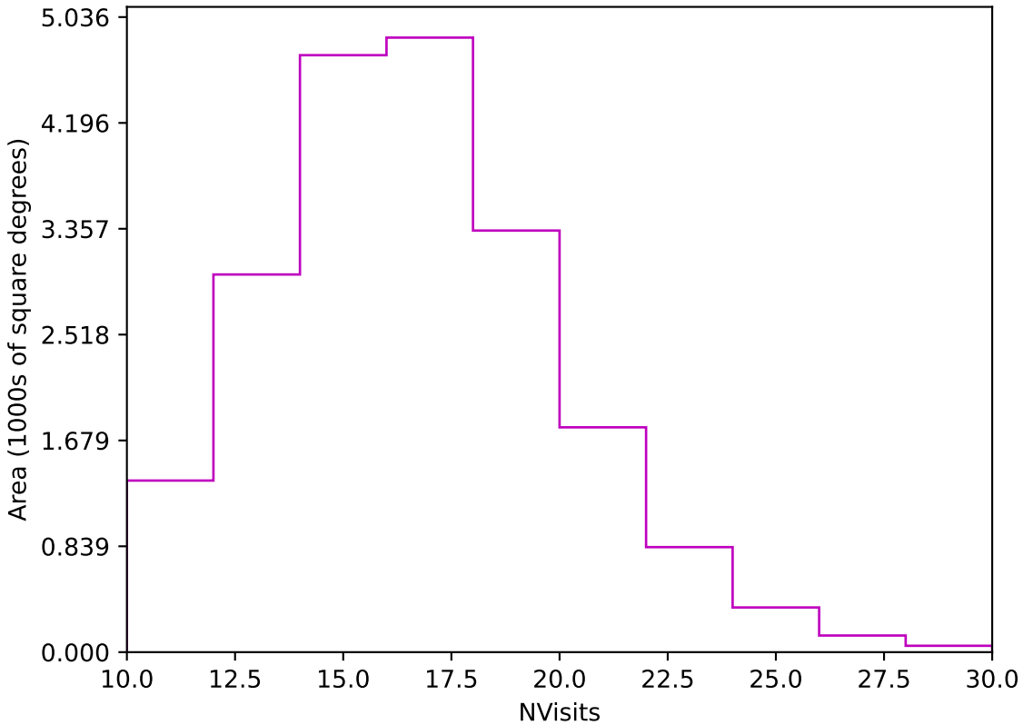
baseline_v3.3_10yrs Yr 1 z band: NVisits
