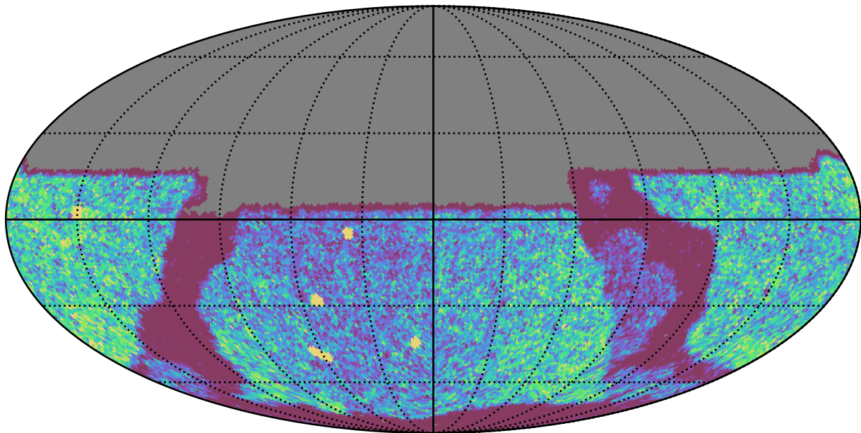
baseline_v3.3_10yrs Yr 1 y band: NVisits
