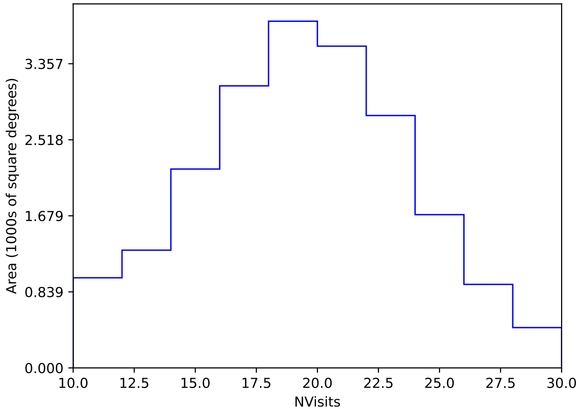
baseline_v3.3_10yrs Yr 1 y band: NVisits
