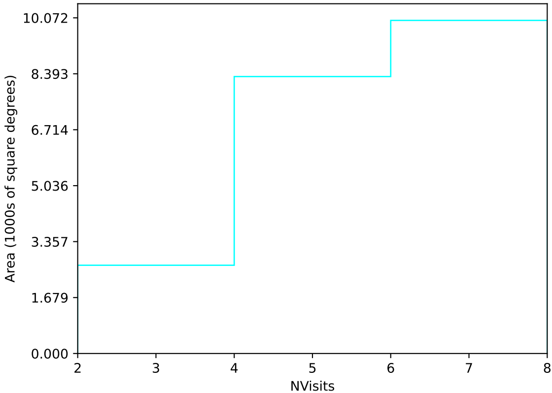
baseline_v3.3_10yrs Yr 1 u band: NVisits
