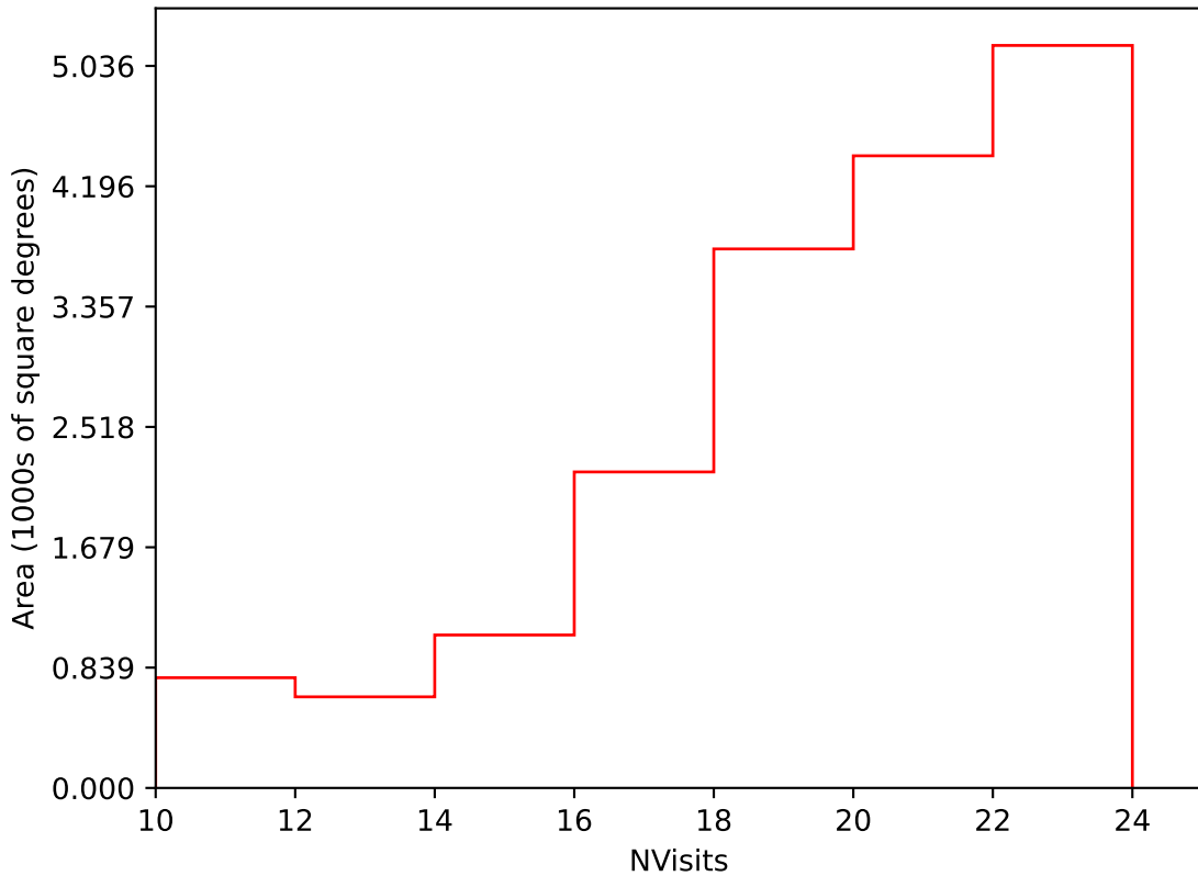
baseline_v3.3_10yrs Yr 1 i band: NVisits
