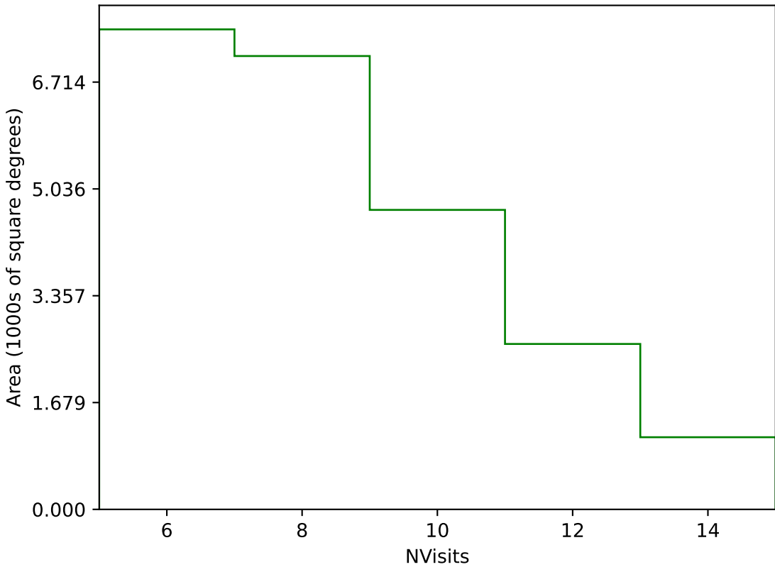
baseline_v3.3_10yrs Yr 1 g band: NVisits
