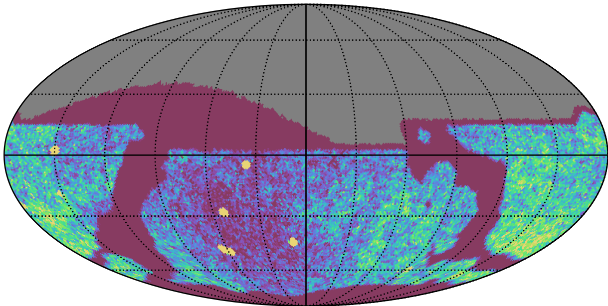
baseline_v3.3_10yrs Yr 1 all bands: NVisits
