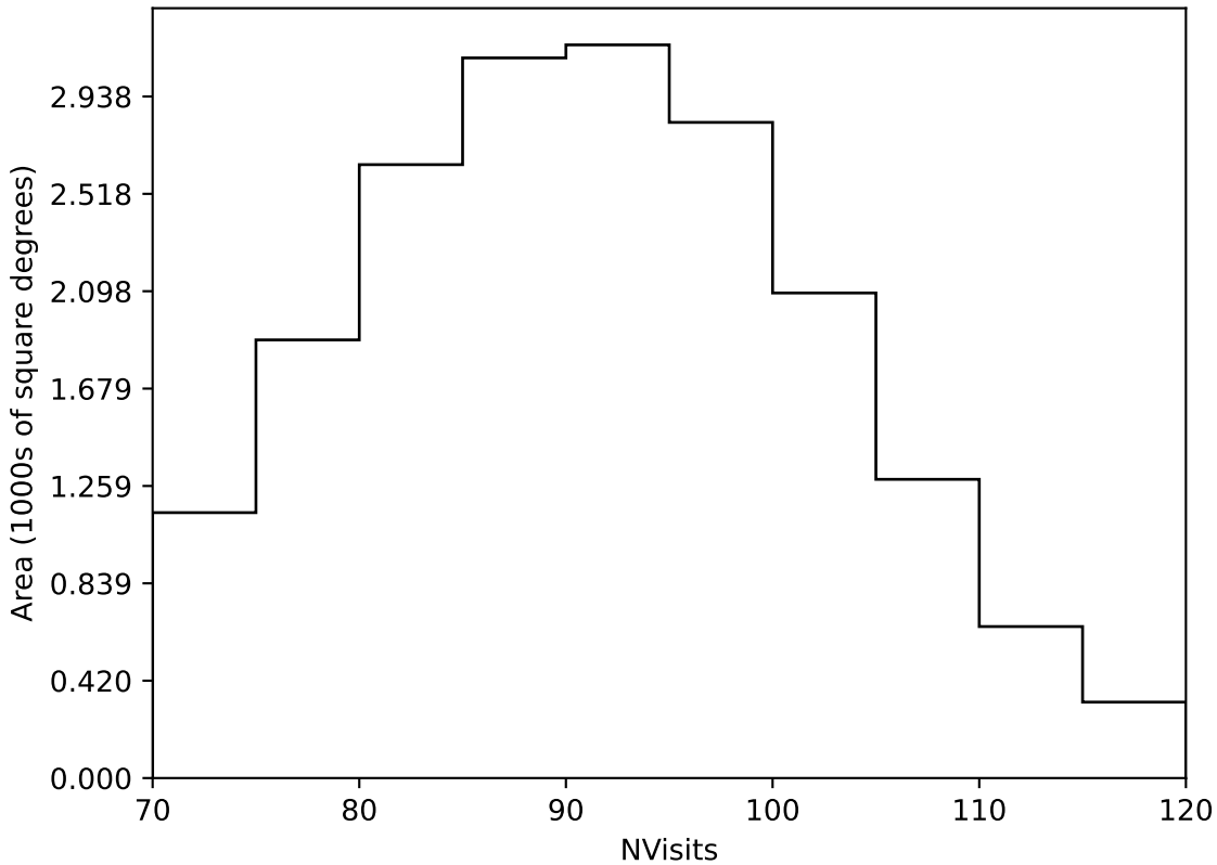
baseline_v3.3_10yrs Yr 1 all bands: NVisits
