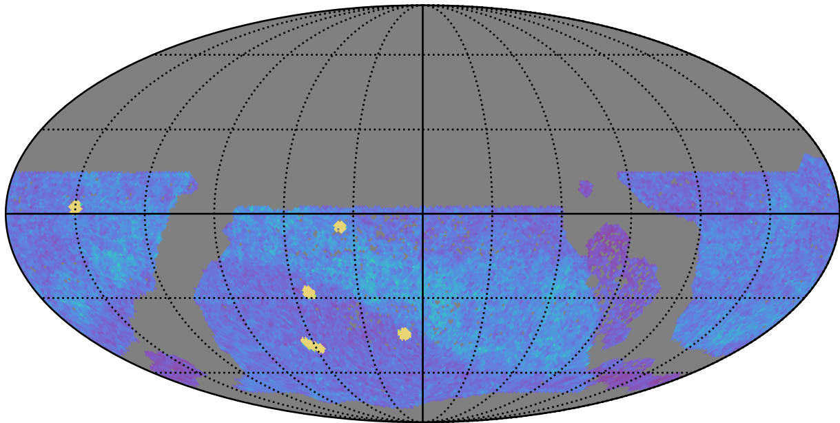
baseline_v3.3_10yrs WFD z band: NVisits
