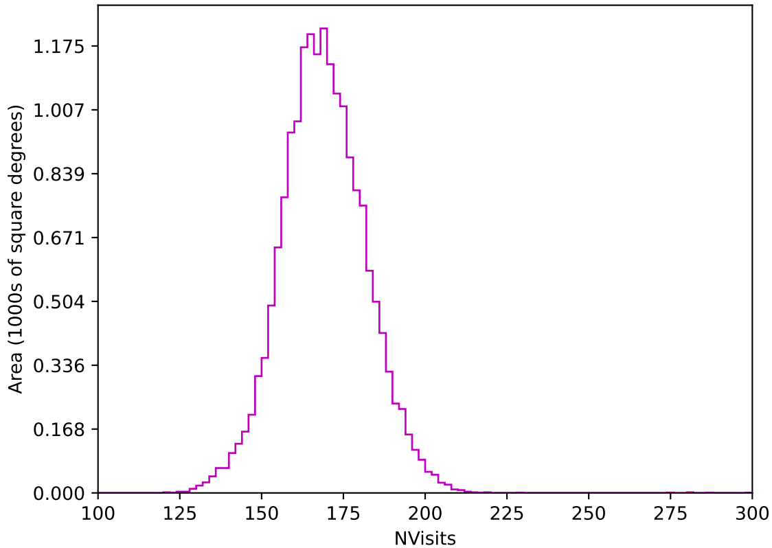
baseline_v3.3_10yrs WFD z band: NVisits
