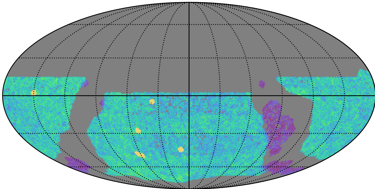
baseline_v3.3_10yrs WFD u band: NVisits
