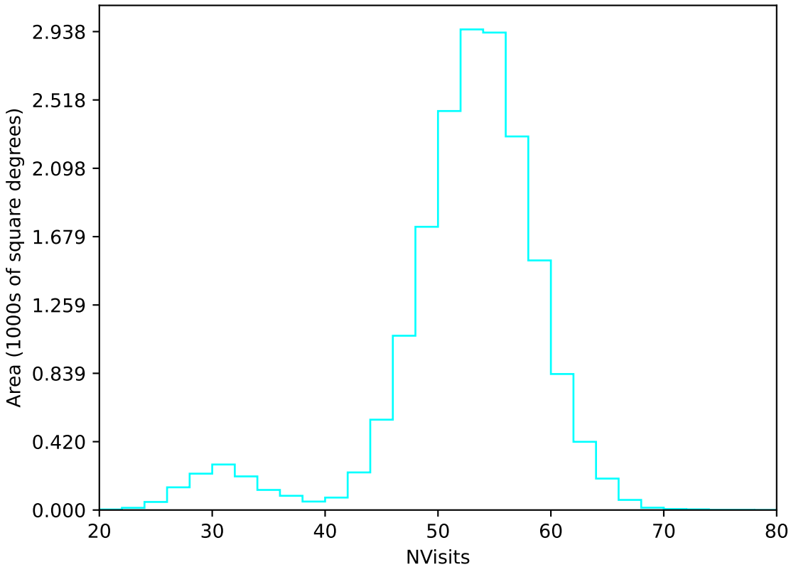
baseline_v3.3_10yrs WFD u band: NVisits
