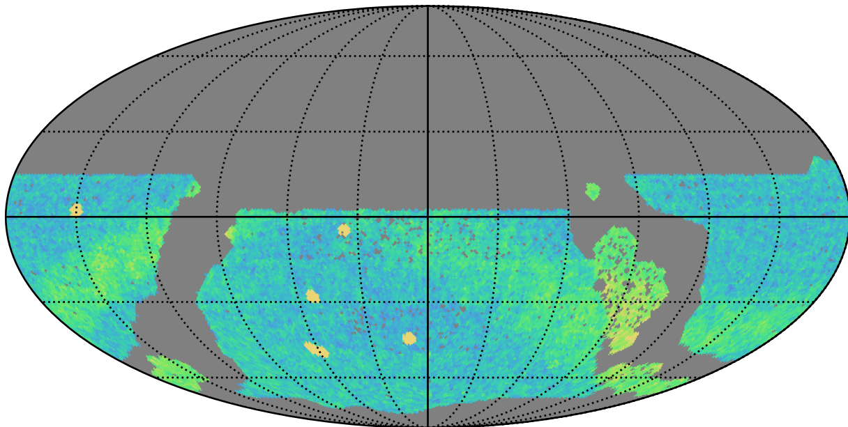
baseline_v3.3_10yrs WFD r band: NVisits
