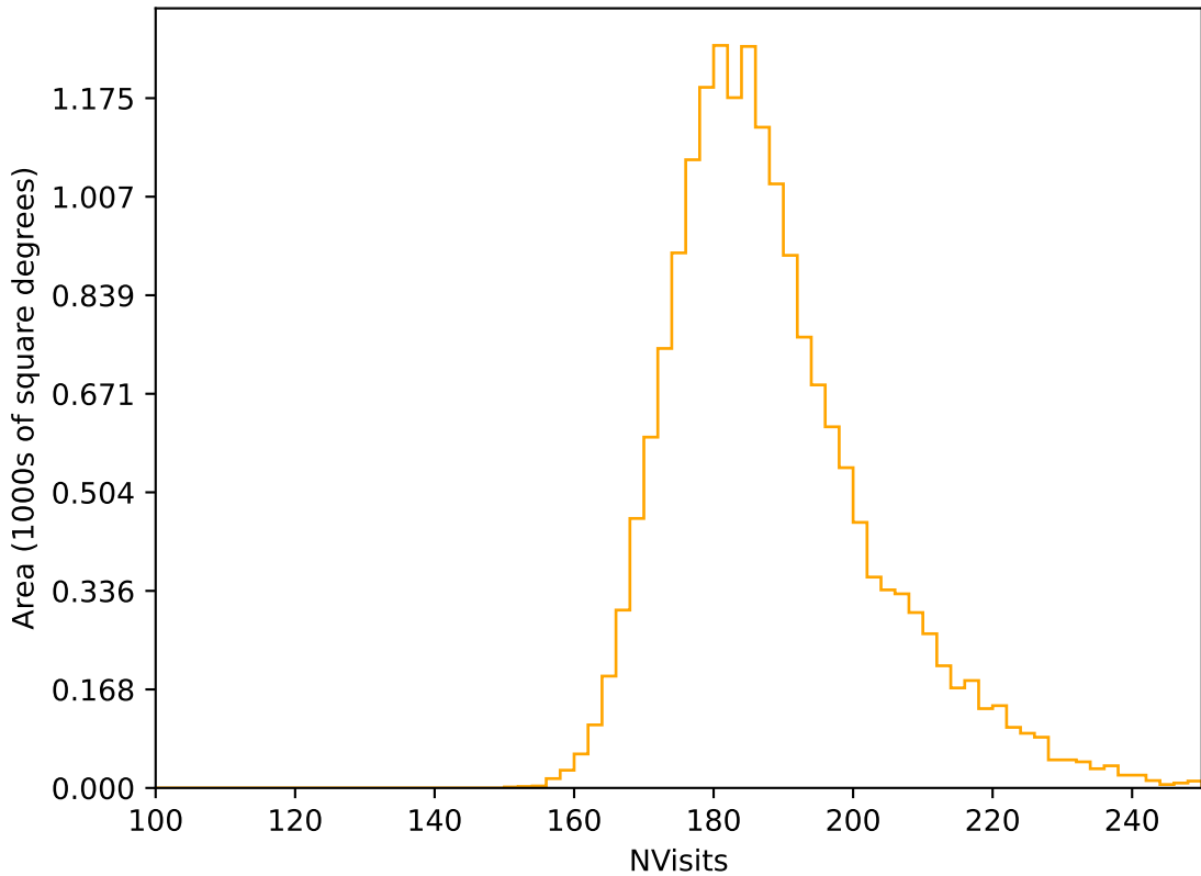
baseline_v3.3_10yrs WFD r band: NVisits
