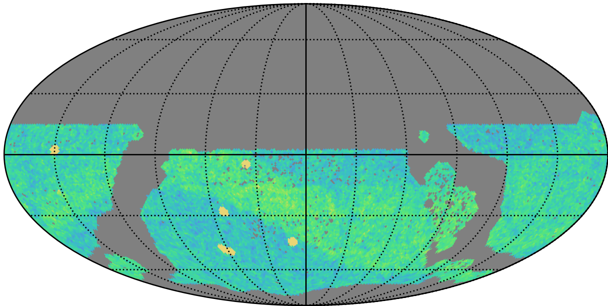
baseline_v3.3_10yrs WFD i band: NVisits
