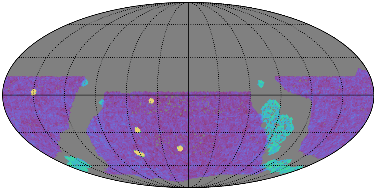
baseline_v3.3_10yrs WFD g band: NVisits
