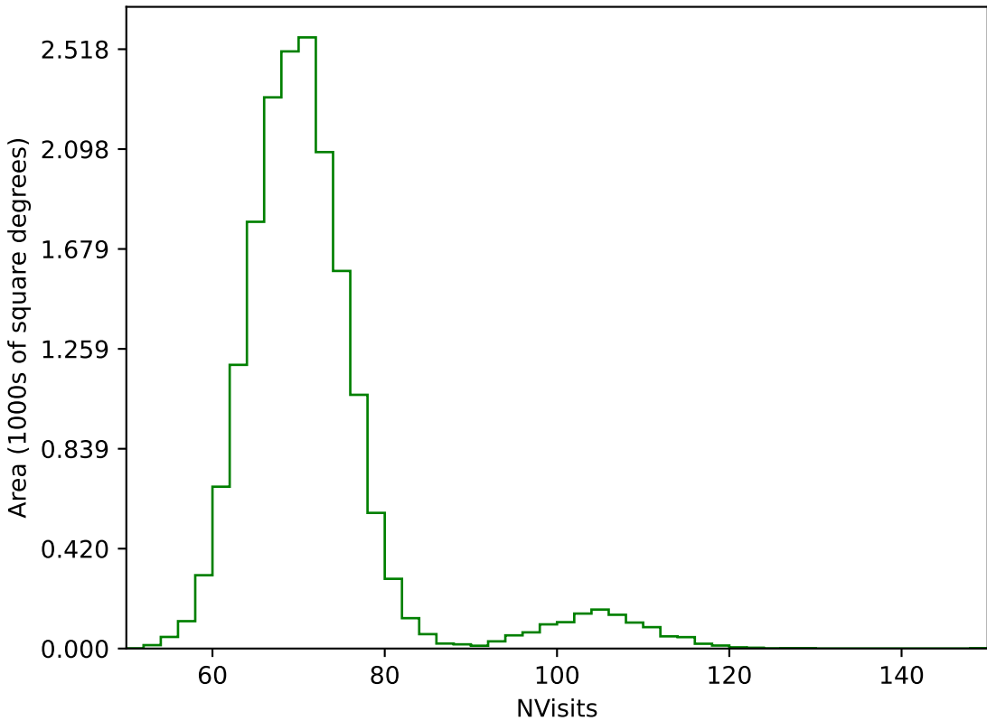
baseline_v3.3_10yrs WFD g band: NVisits
