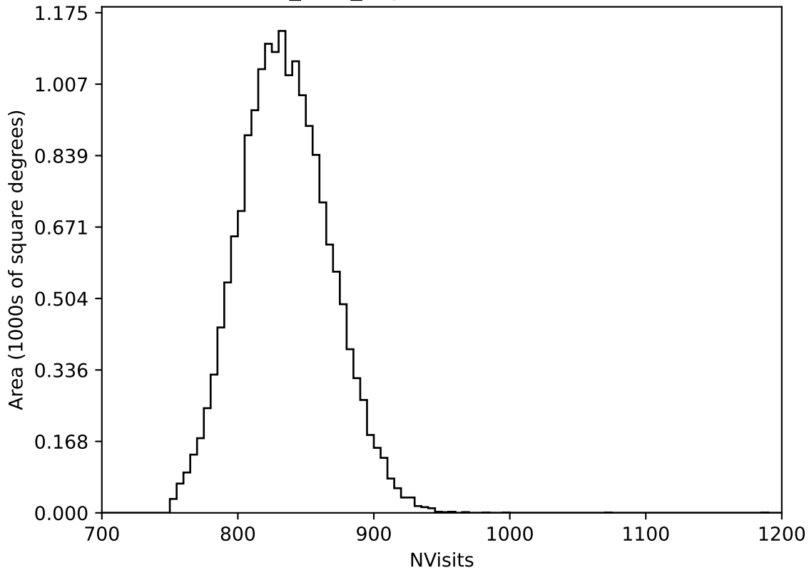
baseline_v3.3_10yrs WFD all bands: NVisits
