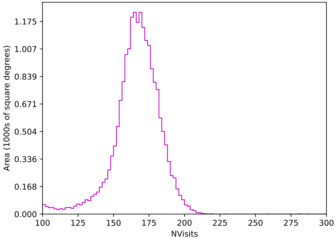
baseline_v3.3_10yrs All sky z band: NVisits
