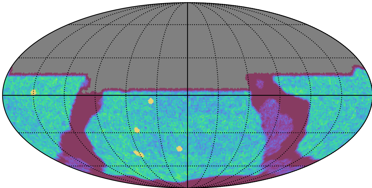
baseline_v3.3_10yrs All sky u band: NVisits
