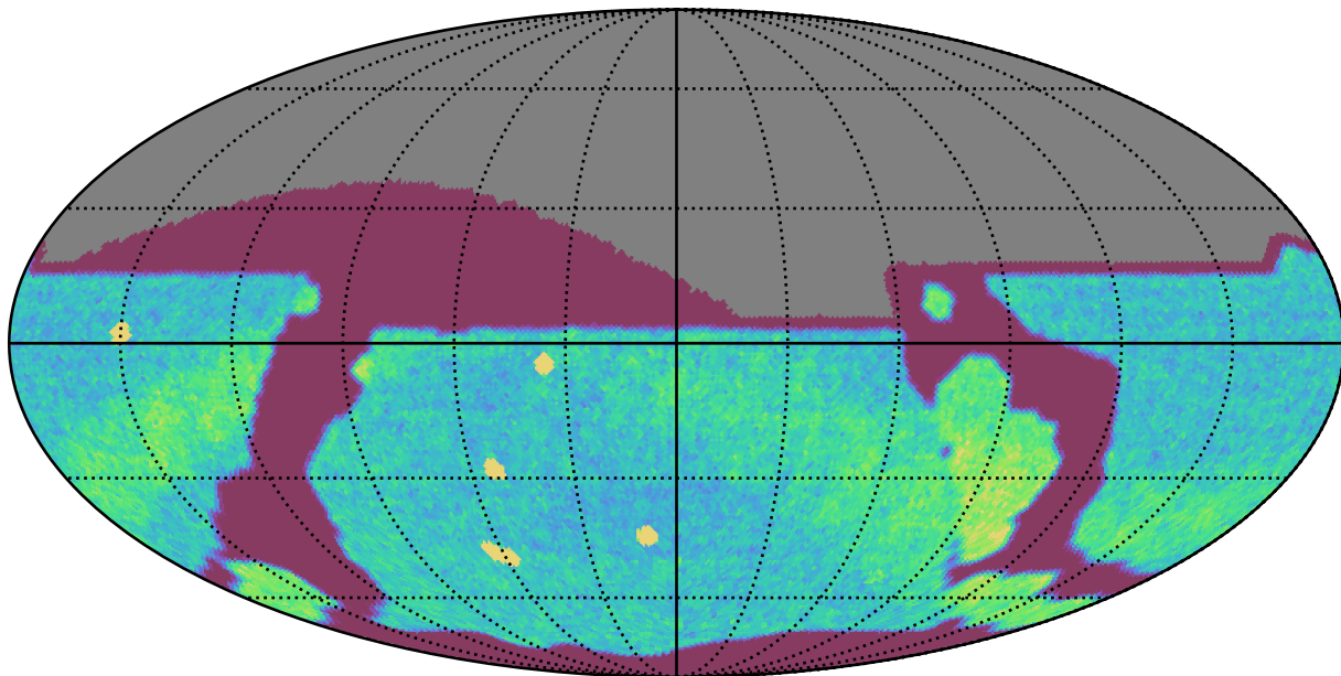
baseline_v3.3_10yrs All sky r band: NVisits
