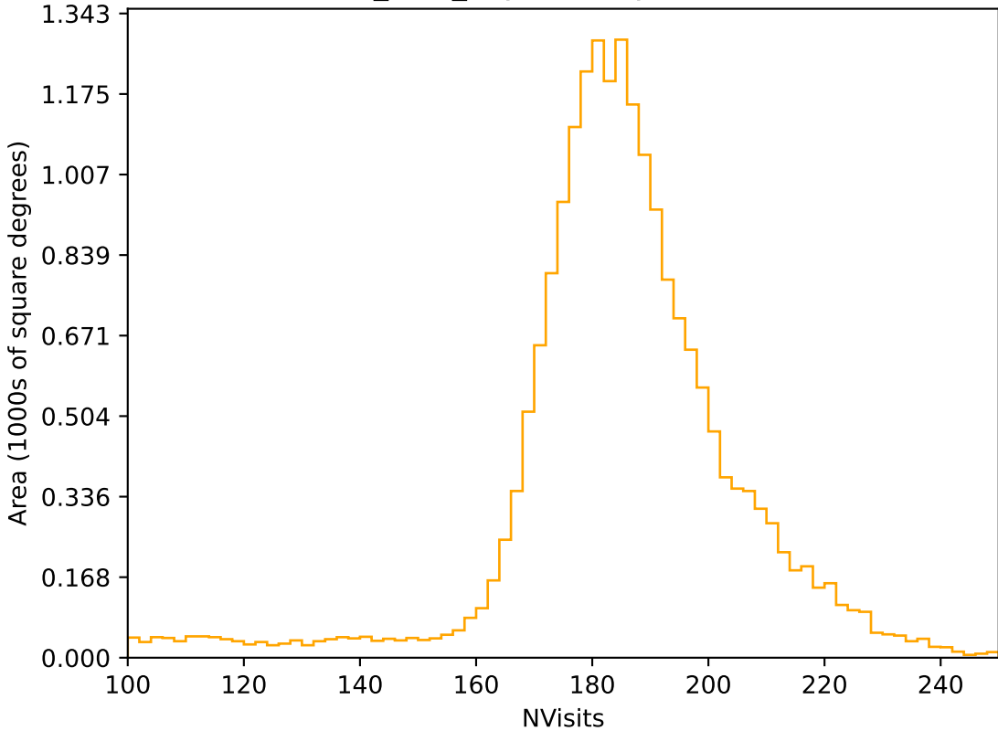
baseline_v3.3_10yrs All sky r band: NVisits
