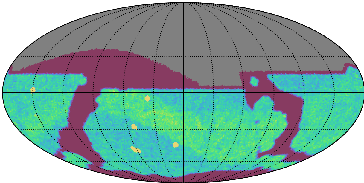
baseline_v3.3_10yrs All sky i band: NVisits
