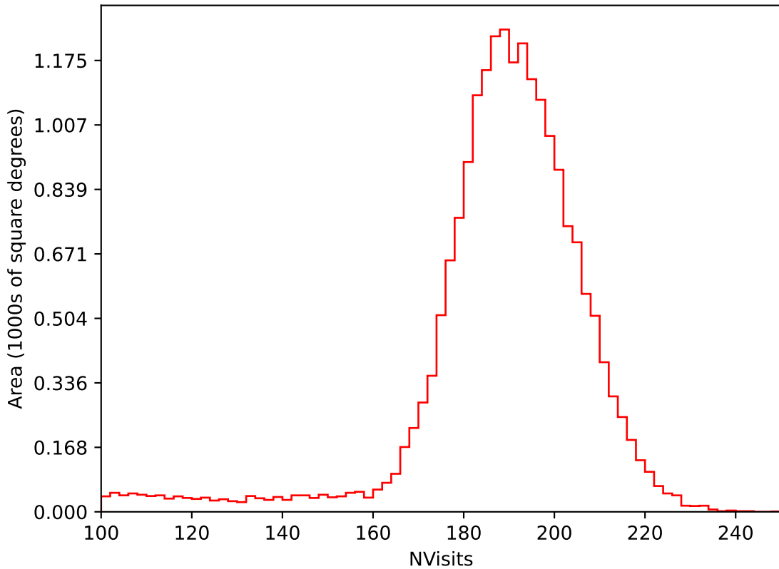
baseline_v3.3_10yrs All sky i band: NVisits
