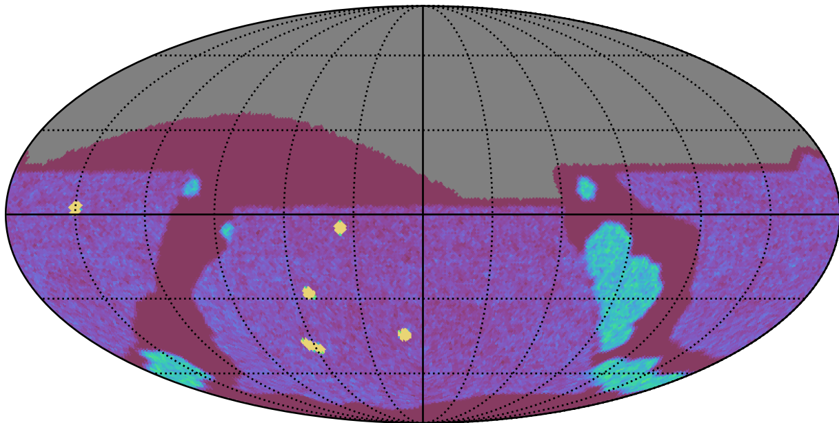
baseline_v3.3_10yrs All sky g band: NVisits
