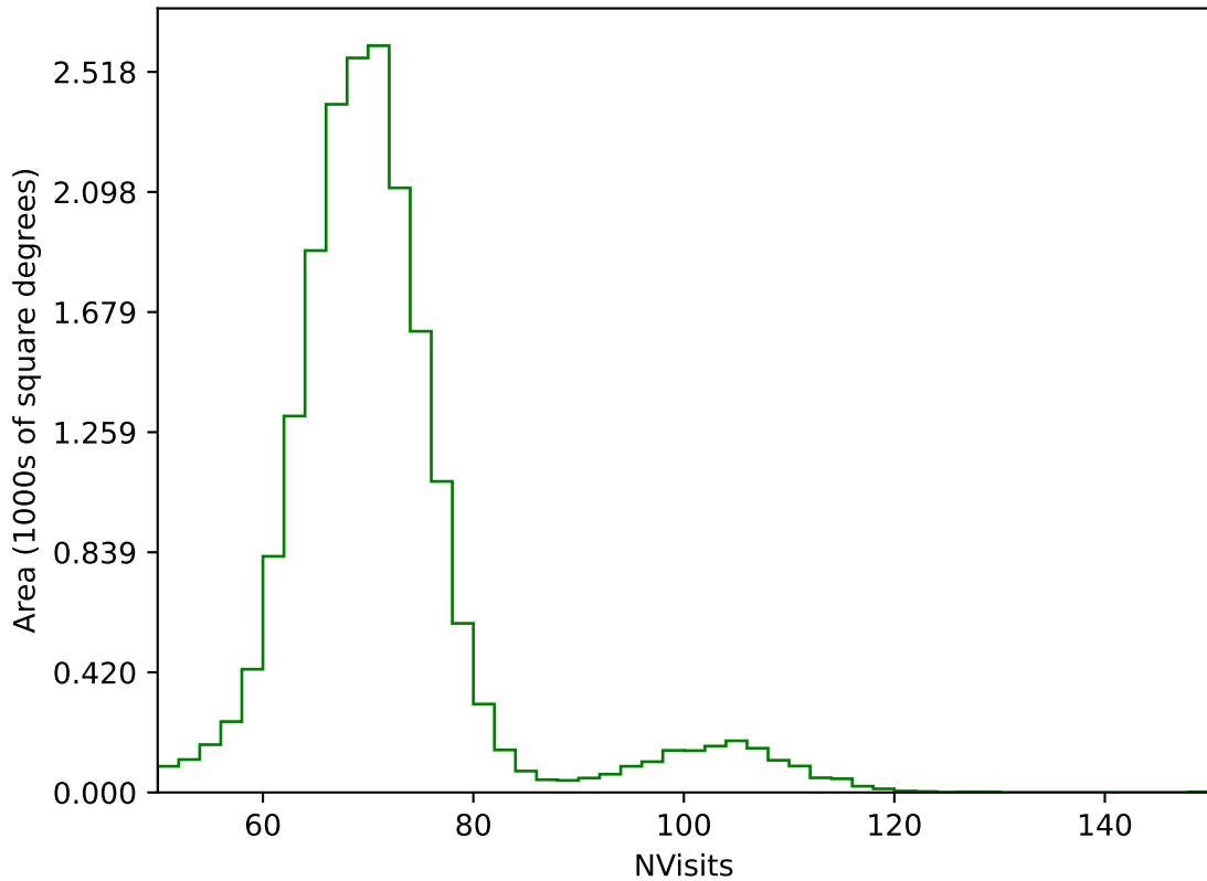
baseline_v3.3_10yrs All sky g band: NVisits
