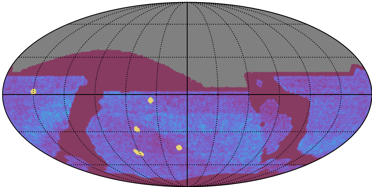
baseline_v3.3_10yrs All sky all bands: NVisits
