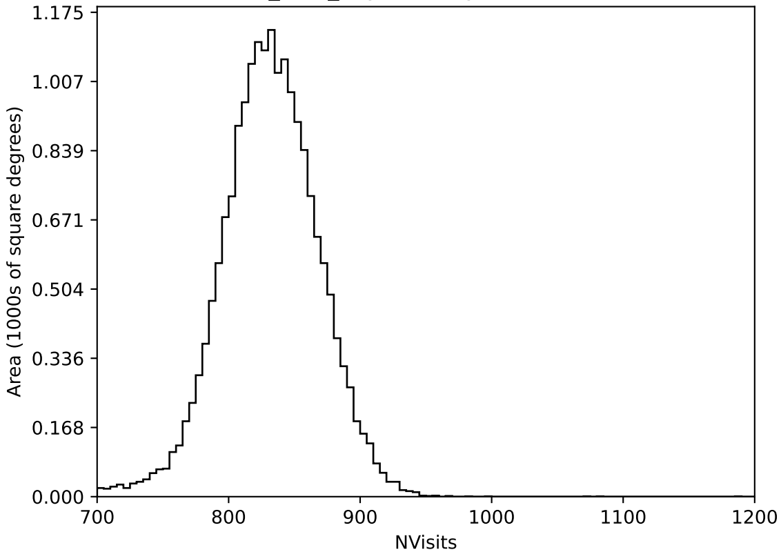
baseline_v3.3_10yrs All sky all bands: NVisits
