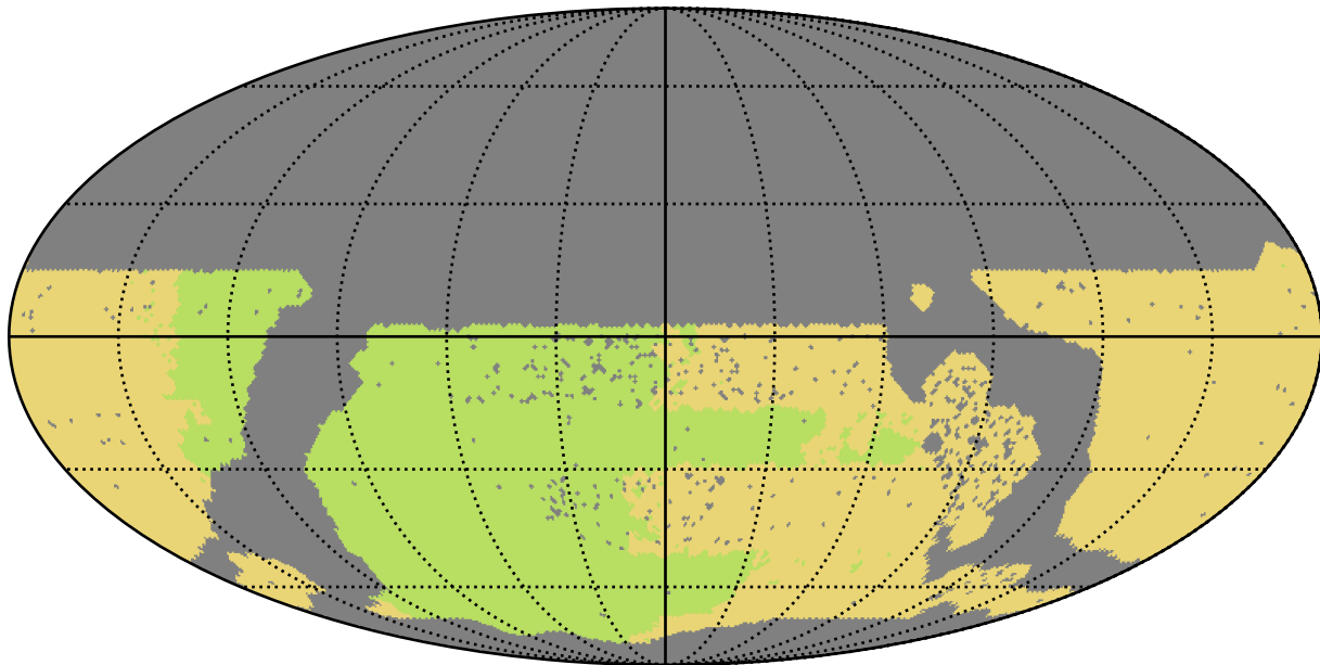
baseline_v3.3_10yrs WFD all bands: NSeasons
