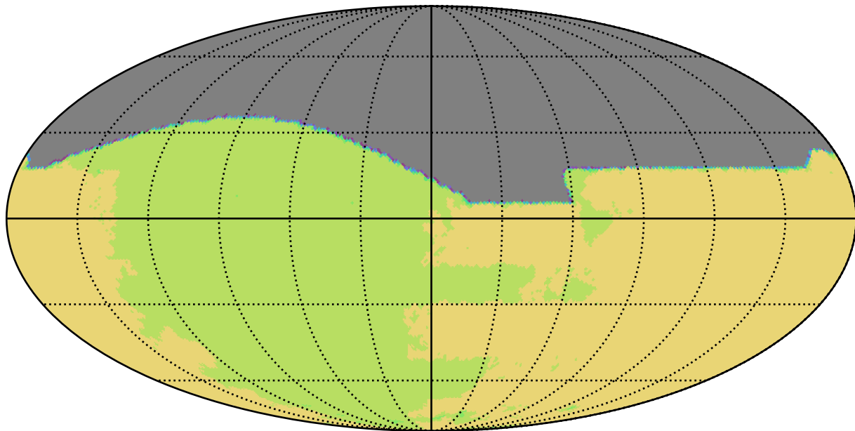
baseline_v3.3_10yrs All sky all bands: NSeasons
