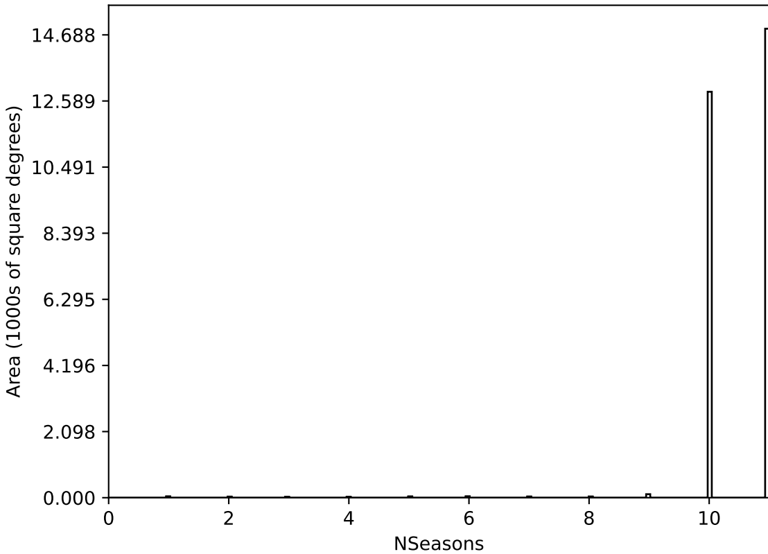
baseline_v3.3_10yrs All sky all bands: NSeasons
