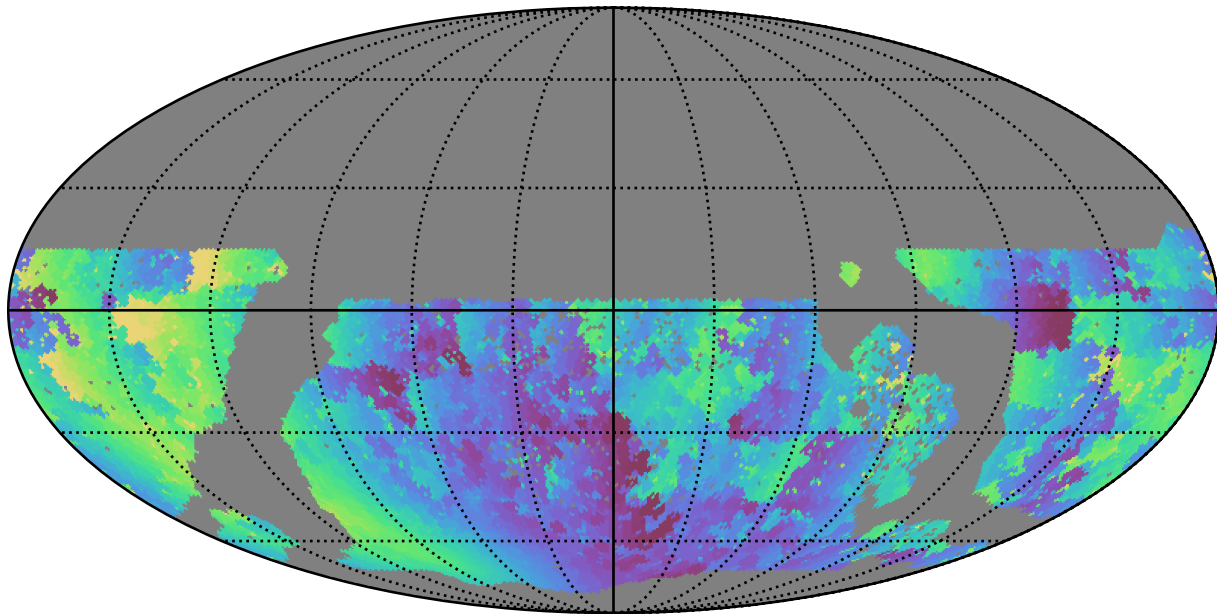
baseline_v3.3_10yrs WFD u band: Min solarElong
